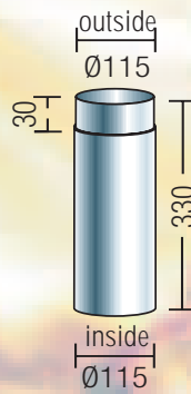
EXTENSION TUBE
