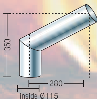
CONNECTING TUBE 60°
