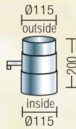
DAMPER TUBE
