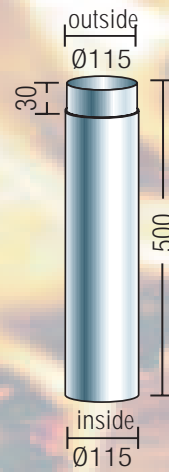
EXTENSION TUBE
