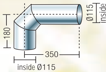
CONNECTING TUBE 90°
